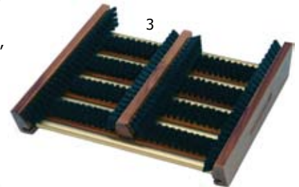
3 Shoe cleaner "Top Classic" Very nice looking shoe cleaner equipped with strong PP-bristles for maximum cleaning effect. Wooden frame work with aluminum parts, size appr. 380 x 360 mm, black bristles No. 190015 piece
